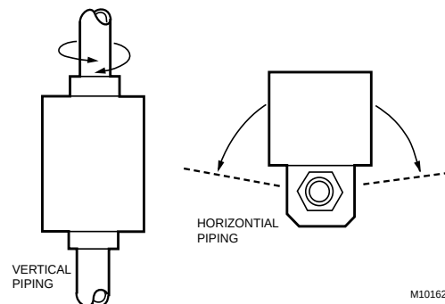
Fig. 5 Mounting positions.
